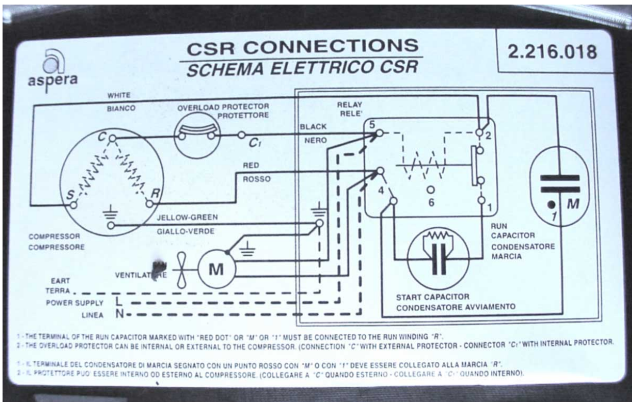
Connections Diagramm
